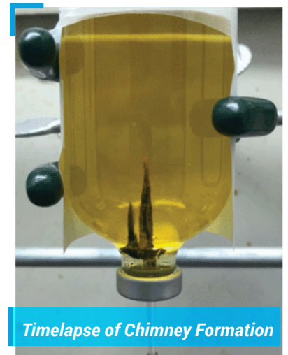
A time-lapse video of a miniature hydrothermal chimney forming in the lab, as it would in early Earth's ocean. Credits: NASA/JPL-Caltech/Flores
